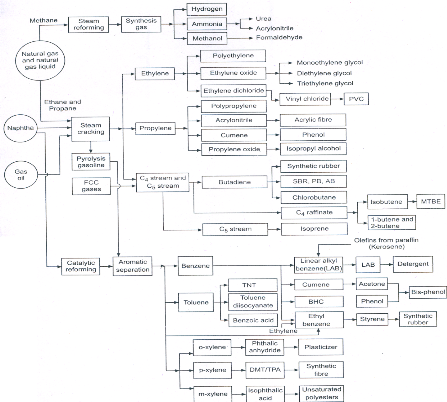
Overall View of a Petrochemical Complex
